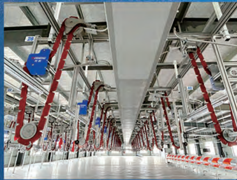
FZDG-2 服装链式智能吊挂 FZDG-2 Clothing Chain Intelligent Hanger
