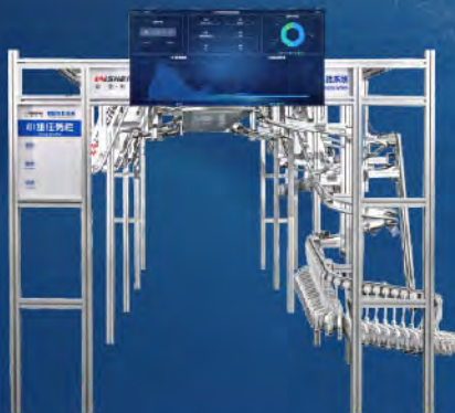
FZDG-1 服装智能吊挂系统 FZDG-1 Clothing smart hanging system
