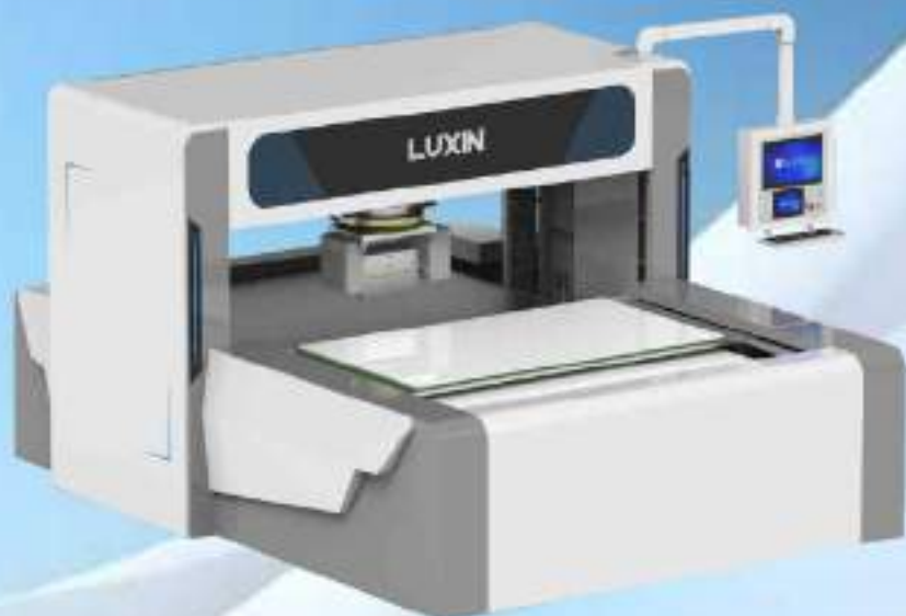
LX-125CS单头双刀双板循环自动裁断机 Single-head double-knife double-board cycle automatic cutting machine
