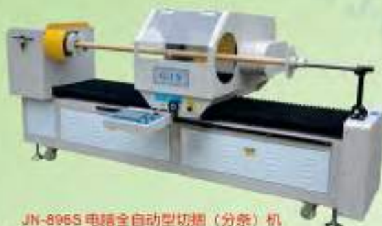
JN-896S 电脑全自动型切排(分条)机 Computer Full Automatic Cutting (Slitter) Machine ( It suitable for cutting fabric, chemical fabric, rubberized fabric, adhesive tape, leather, paper, interlining, etc. )
